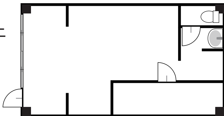
間取
